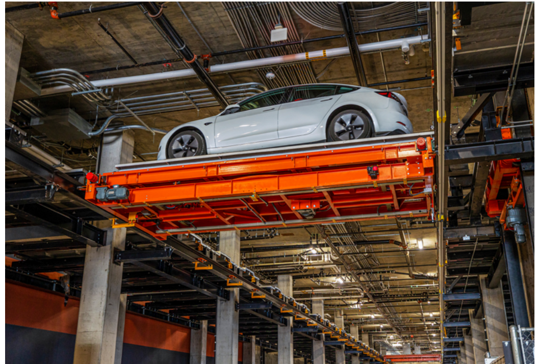
233-space Fully Automated Parking Solution During System Commissioning
